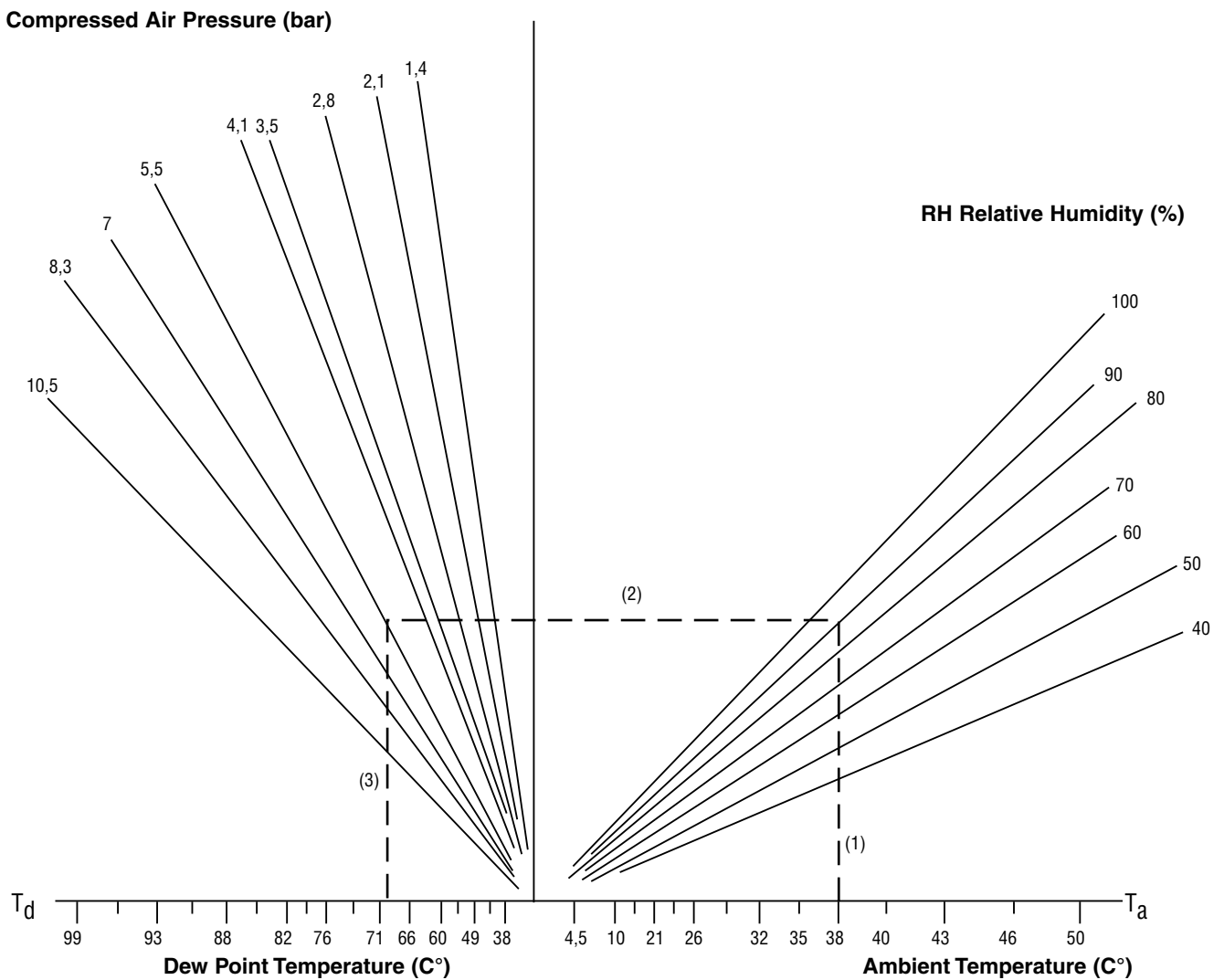
Nomograph Estimates Dew Point of Compressed Air
