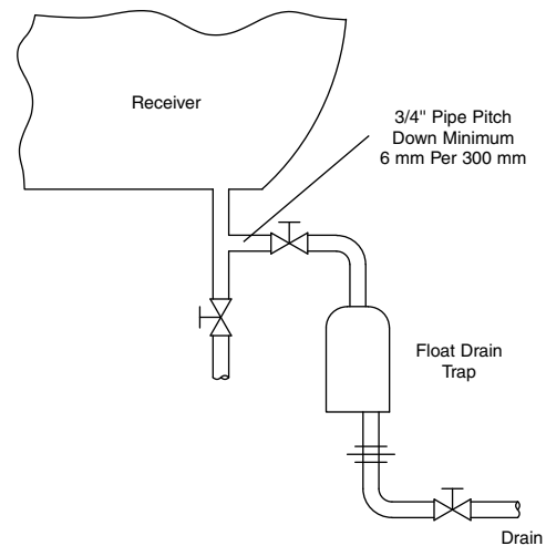
Figure LD-435-2. Install the drain trap on side to get better access or compensate for lack of space under the receiver (particularly for drain trap used under compressors).
