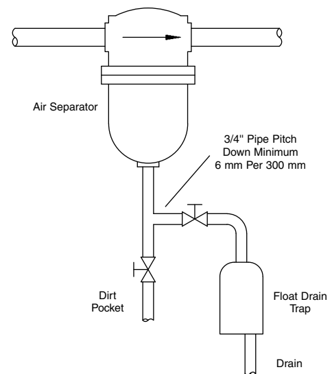
Figure LD-433-2. Installation of a drain trap on side of separator.
