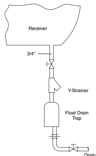
Figure LD-435-4. Same installation but with a strainer protecting the drain trap.
