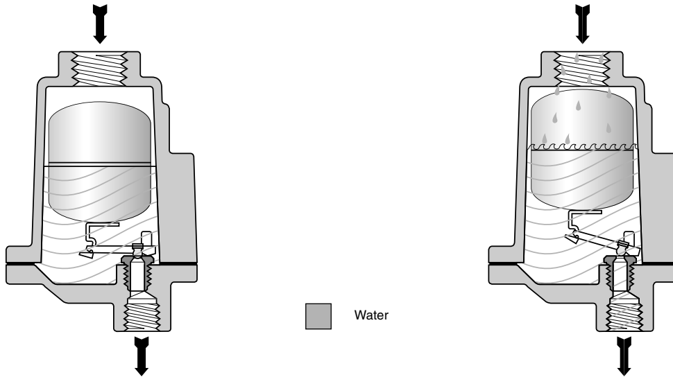
Figure LD-422-1. Operation of the Model 1-LD Free Floating Lever Drain Trap As water begins to fill the body of the trap, the float rises, opening the discharge valve. Motion of the free floating valve lever is guided to provide precise closure.
