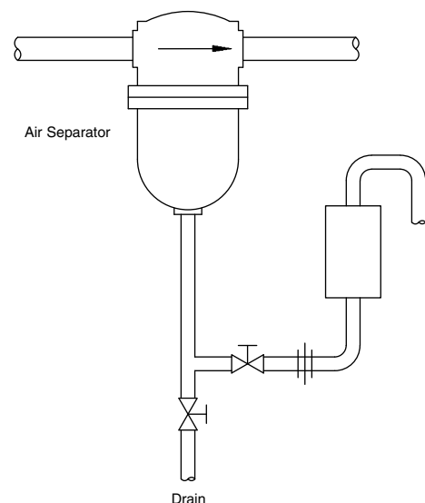
Figure LD-431-2. 800 Series inverted bucket drain trap installed on compressed air contaminated by oil.
