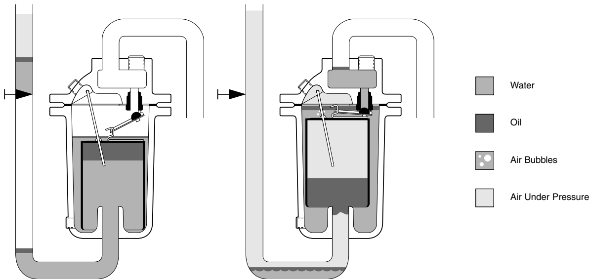
Figure LD-420-1. Operation of the BVSW Inverted Bucket Drain Trap
