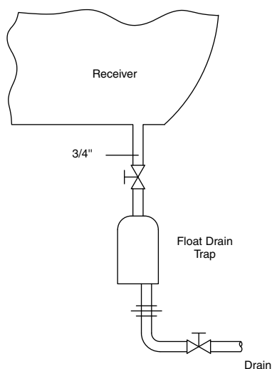
Figure LD-435-3. Installation not recommended because of the dirt problem that can occur with a drain trap installed straight under the receiver.
