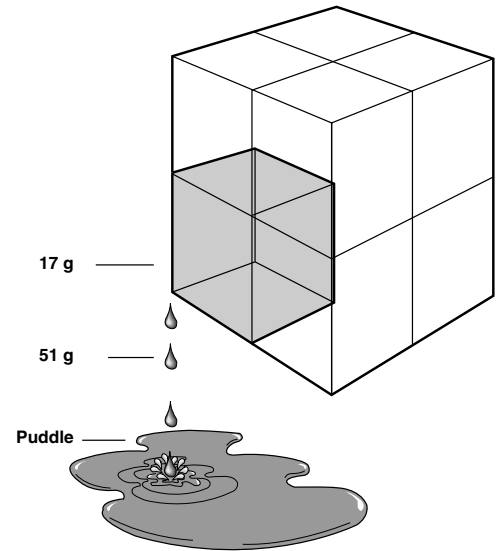
Figure LD-417-3. Pressure: 8 bar(a) Temp: 20°C Air = 1 m 3 Moisture = 68 g Max Possible = 17 g 51 g of Liquid
